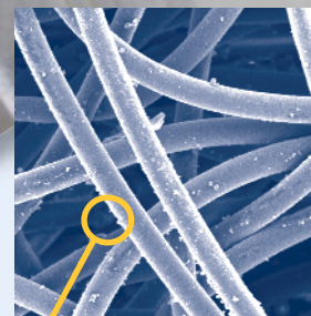
Dura-Life Hydroentangled Media 10 Micron Particulate at 600%
