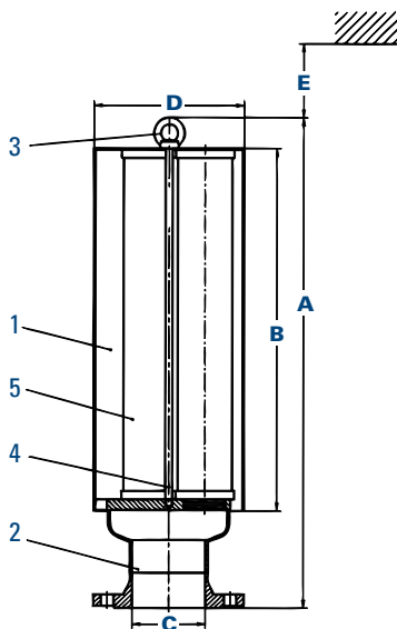
Vent Filter with ANSI Flange Connection
