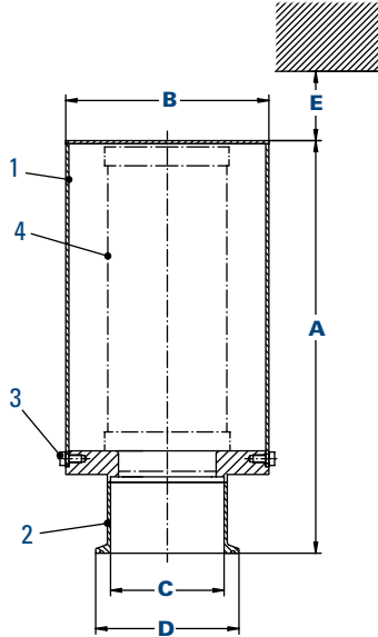
Vent Filter with Tri-Clamp Connection
