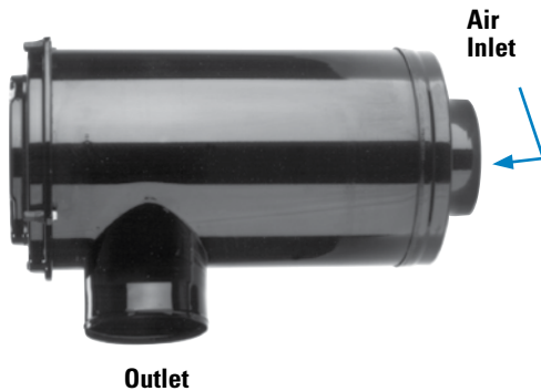
Because of the cone-shaped filter inside the housing, EBA Konepac™ is smaller in size compared to the ERA without sacrificing airflow. This allows trucks to meet width requirements in all states.
