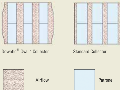
Cross-sectional area of collector dirty air.
