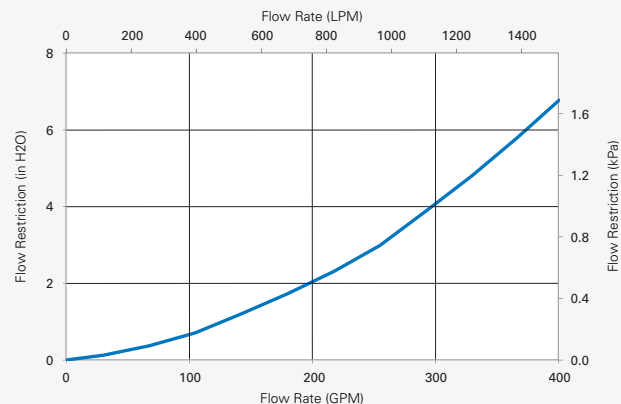
T.R.A.P. Breather
