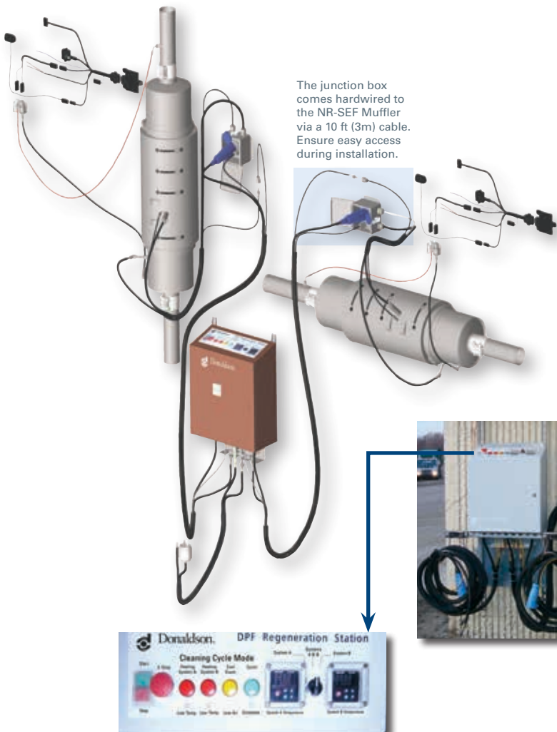
Donaldson DPF Regeneration Station (Part No. X009584) with simple, automated control panel.
